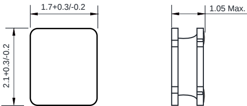
Dimensions: [mm]
